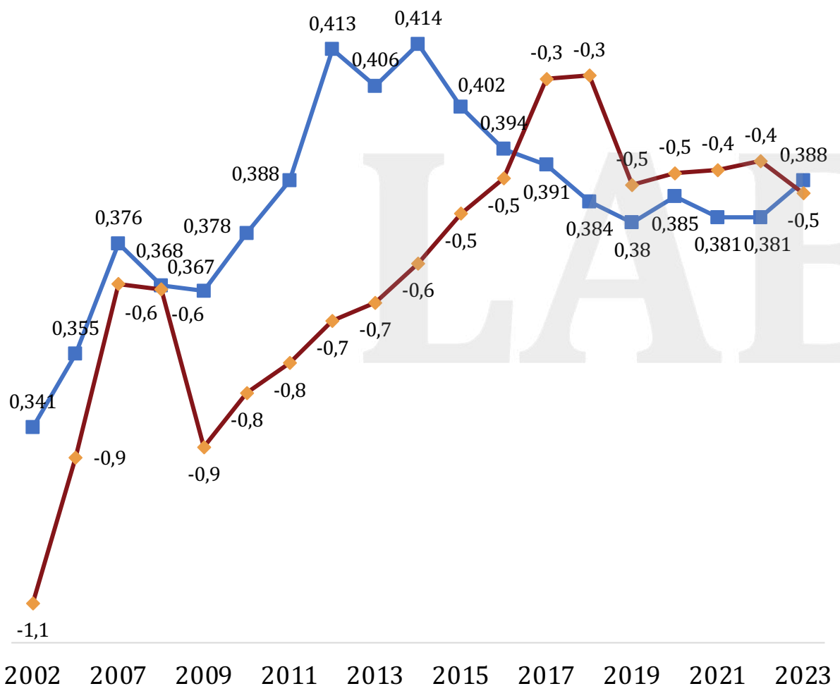
Rasio Gini Control of Corruption
